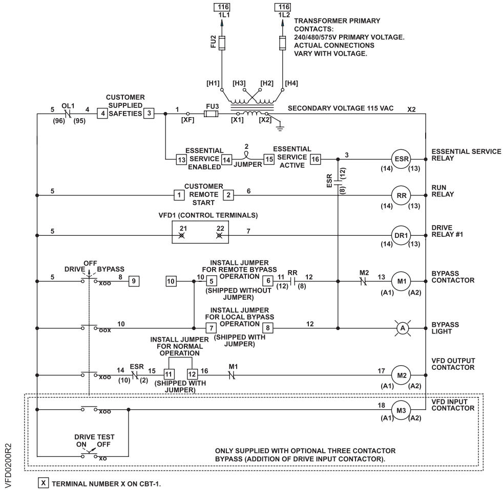
Figure 2. C-Bypass 120 Vac Control Circuit.
