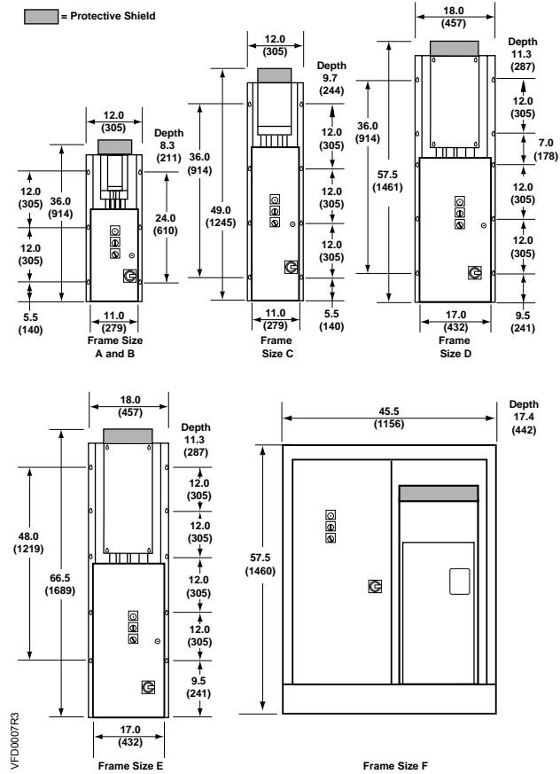
Figure 1. C-Bypass Dimensions in Inches (cm).
