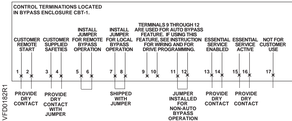
Figure 4. C-Bypass Terminations.
